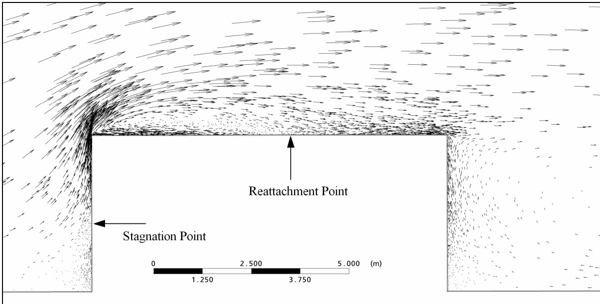
Figure 5: Velocity profile around the building for the finest grid with the numerical prediction of the stagnation point and reattachment location identified.
