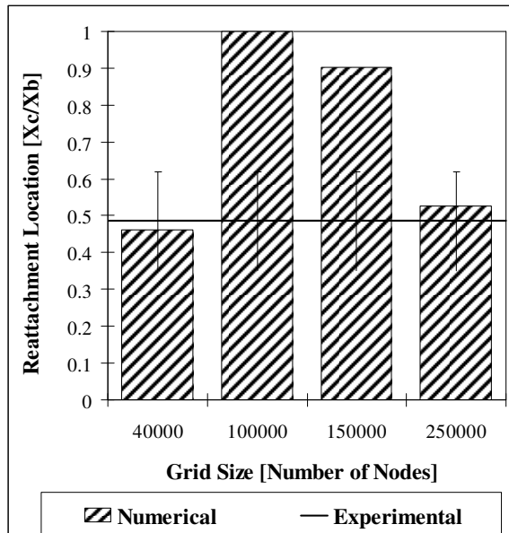
Figure 4: Non-dimensional reattachment locations on the roof of the building where X_c is the reattachment location and X_b is the building depth. Error bars indicate the experimental variation.
