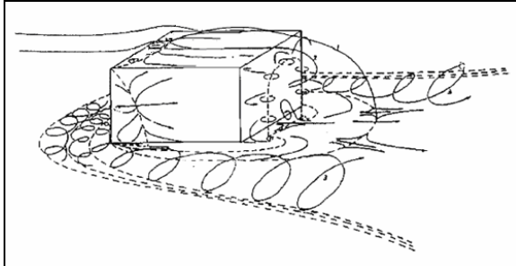
Figure 1: General flow visualization with flow normal to building face. [1]
