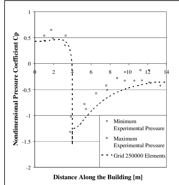
Figure 6: Pressure distribution over the building for the finest grid compared to experimental data.
