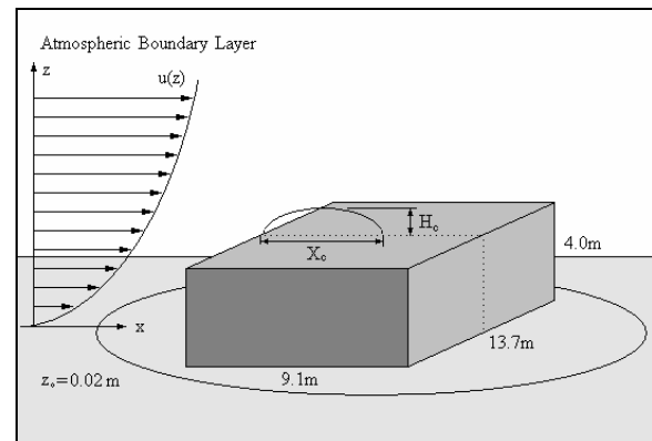
Figure 2: Building configuration with separation bubble defined.
